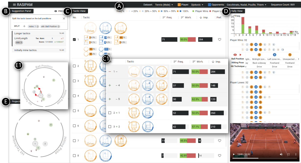
Fig. 1. A screenshot of our system for interactive tactic mining. Domain experts first need to select a player of interest on the control bar (A) to analyze his/her tactics. Then the system mines a initial set of tactics and visualizes them through intuitive glyphs in the Tactic View (C). Meanwhile, the Project View (E) provides an overview of the tactics through a semantic projection method, allowing domain experts to quickly understand the tactics. Experts are then allowed to give suggestions to improve the tactics based on their domain knowledge in the Suggestion Panel (B). The system will refine the tactic set and compare the new tactics with the original ones (C1 and E1). For detailed exploration, the Rally View (D) shows more details about a chosen tactic, including a bar chart displaying where the tactic is used, a list of all rallies involving the tactic, and a video player for the video segment of each rally.
