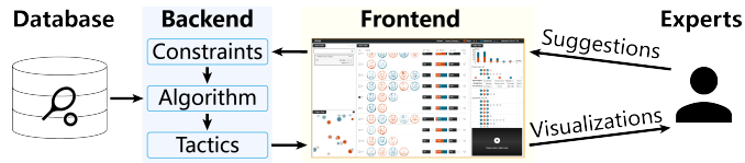
Fig. 3. Our system architecture for interactive tactical analysis.
