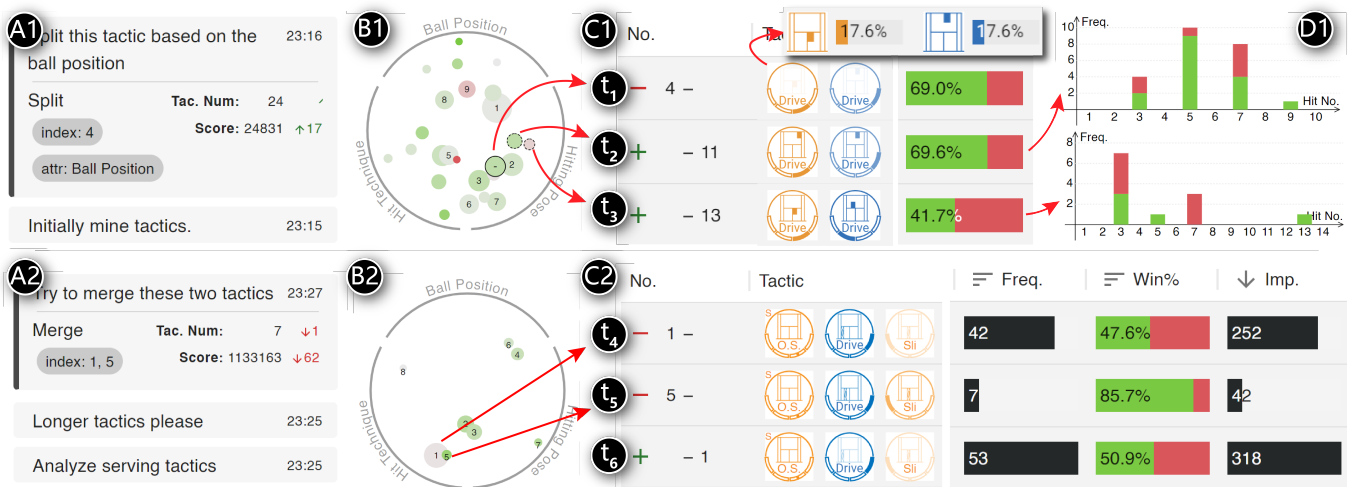
Fig. 9. Screenshots of the tennis case, where experts split a seesaw-battle tactic (A1-D1) and merged two serving tactics (A2-C2). We present the screenshots of Suggestion Panel (A1, A2), Projection View (B1, B2), Tactic View (C1, C2), and the stacked bar chart in Rally View (D1).
